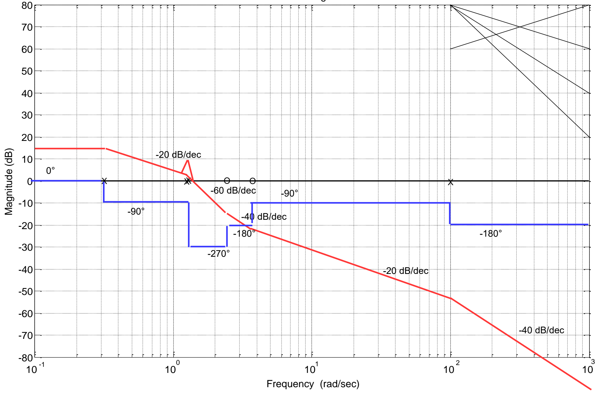
Bode Diagram
